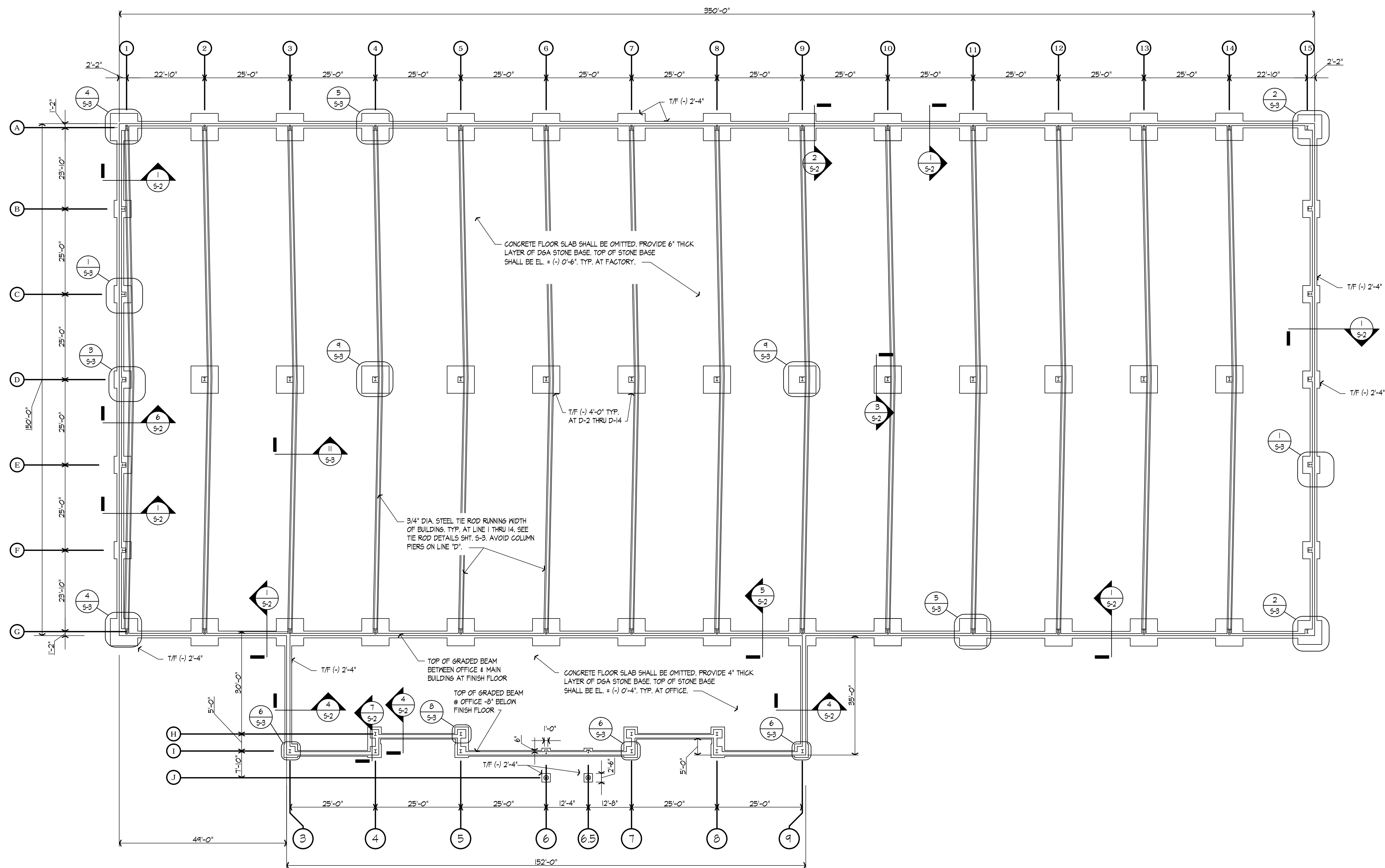
FOUNDATION PLAN SCALE: 1/16" = 1' - 0"
